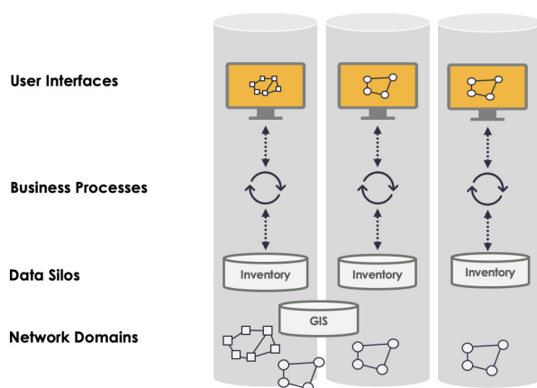
Figure 4: Typical accumulation of siloed inventory systems at a service provider
